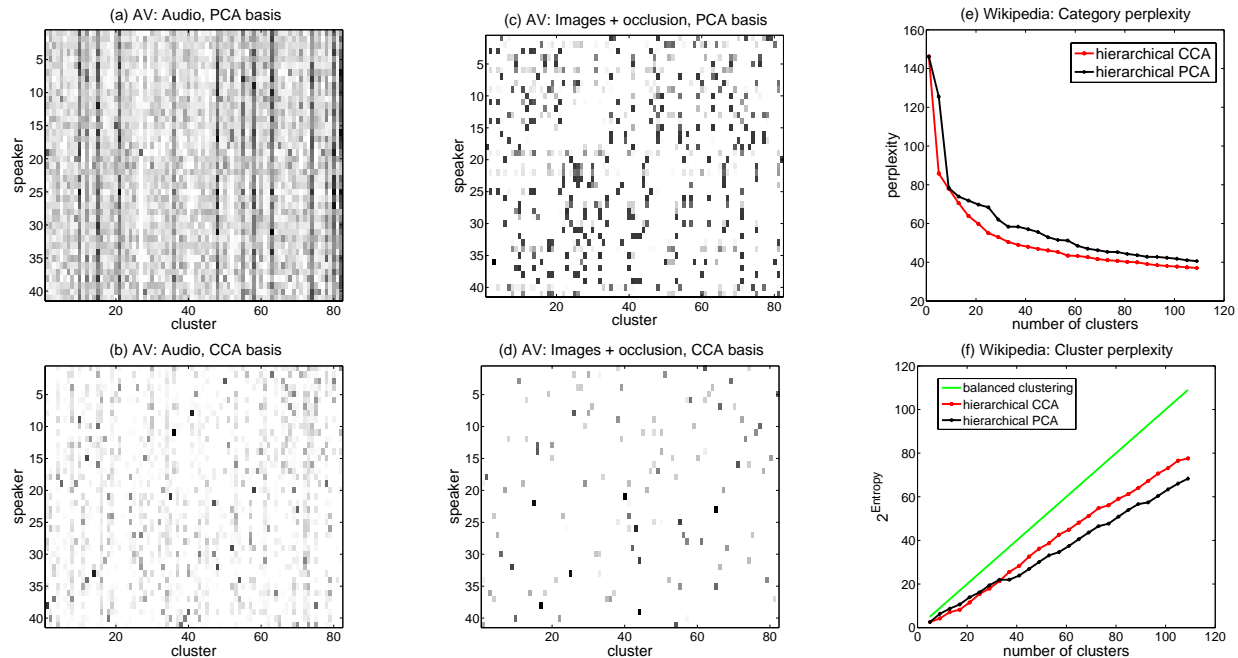
Figure 1. (a-d) Distributions of cluster assignments per speaker in audio-visual experiments. The color of each cell (s, c) corresponds to the empirical probability p(c|s) (darker = higher). (e-f) Wikipedia experiments: (e) Conditional perplexity of article category given cluster, 2^{H(a|c)} , as a function of the number of clusters. (f) Perplexity of the cluster distribution ( 2^{H(c)} ) as a function of the number of clusters.
