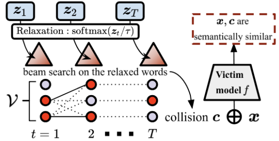
Figure 1: Overview of generating semantic collision \mathbf{c} for a query input \mathbf{x} . The continuous variables z_t relax the words in \mathbf{c} and are optimized with gradients. We search in the simplex produced by z_t for the actual colliding words in \mathbf{c} .
