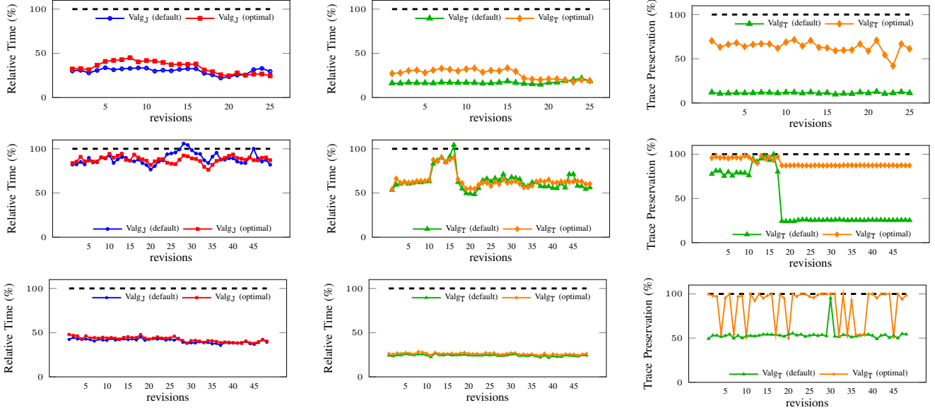
Fig. 6: Effect of hyperparameter tuning on \text{Valg}_J time (left), \text{Valg}_T time (middle), and unique traces checked (right). The projects are cassette-nibbler [52], ASM-NonClassloadingExtensions [34], and jpoker [22], from top to bottom.
