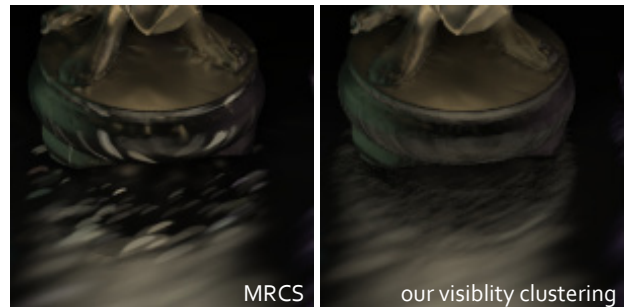
Figure 5: Global light methods. Comparison of matrix-row column sampling (left: 202 seconds) and visibility clustering (right: 213 seconds). Both methods use 200,000 VPLs, and compute only indirect illumination. MRCS selects 10k lights for shadow map evaluation and shading, while visibility clustering uses only 5k shadow maps and shades from all VPLs, yielding less splochy images.
