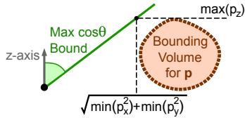
Figure 4: Bounding the minimum angle (and hence maximum cosine) to a bounding volume. See Equation 4.
