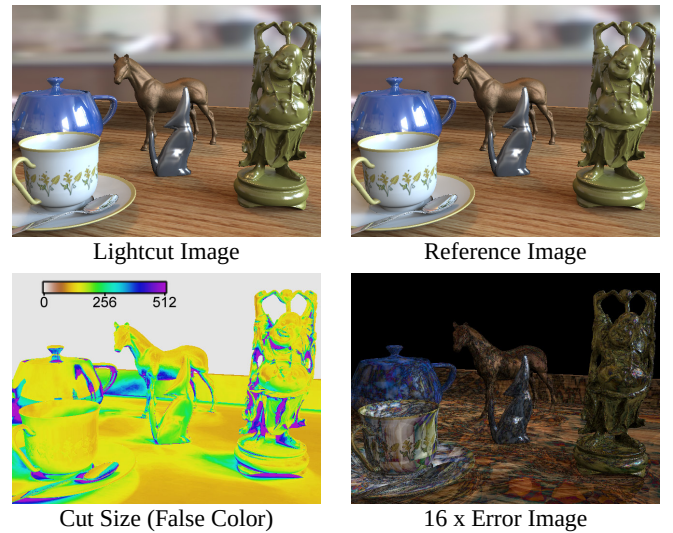
Figure 7: Tableau scene illuminated by an HDR environment map. In parentheses are averages over only pixels containing geometry.
