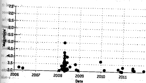
FIGURE 5-4D: EARTHQUAKES NEAR RENO, NEVADA JANUARY 1, 2006–DECEMBER 31, 2011
