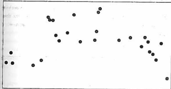
FIGURE 5-6A: LIMITED SAMPLE OF DATA
