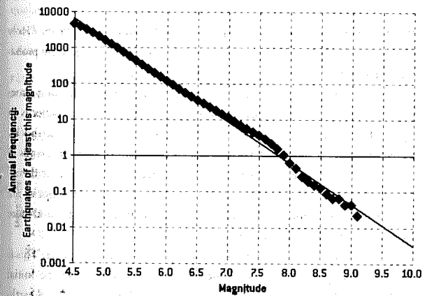
FIGURE 5-3B: WORLDWIDE EARTHQUAKE FREQUENCIES, JANUARY 1964–MARCH 2012, LOGARITHMIC SCALE
