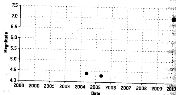
FIGURE 5-4C: EARTHQUAKES NEAR LÉOGÂNE, HAITI JANUARY 1, 2000–JANUARY 12, 2010
