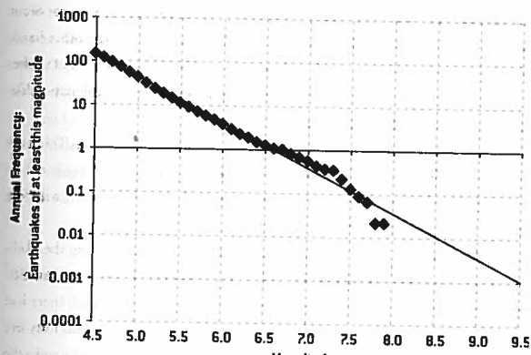
FIGURE 5-7B: TŌHOKU, JAPAN EARTHQUAKE FREQUENCIES GUTENBERG-RICHTER FIT
