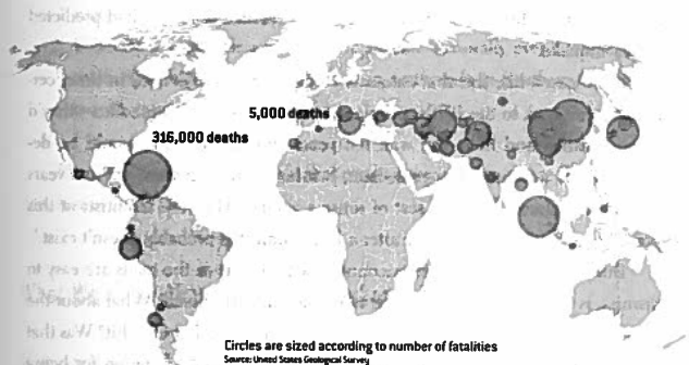
FIGURE 5-1: DEADLIEST EARTHQUAKES SINCE 1900
