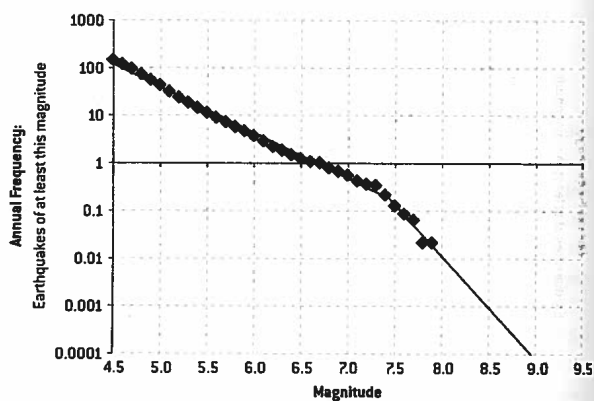
FIGURE 5-7C. TŌHOKU, JAPAN EARTHQUAKE FREQUENCIES CHARACTERISTIC FIT
