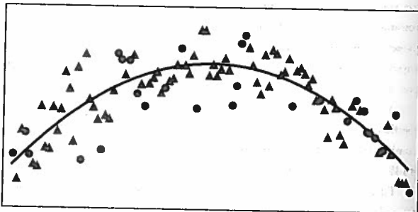
FIGURE 5-5: TRUE DISTRIBUTION OF DATA
