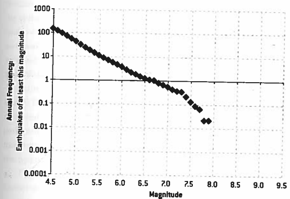
FIGURE 5-7A: TŌHOKU, JAPAN EARTHQUAKE FREQUENCIES JANUARY 1, 1964–MARCH 10, 2011
