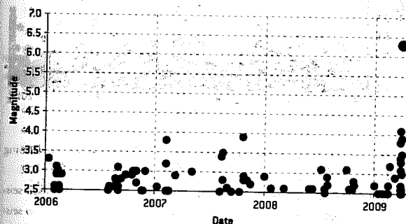
FIGURE 5-4A: EARTHQUAKES NEAR L’AQUILA, ITALY JANUARY 1, 2006–APRIL 6, 2009
