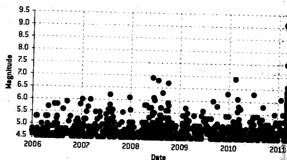
FIGURE 5-4B: EARTHQUAKES NEAR TÔHOKU, JAPAN JANUARY 1, 2006–MARCH 11, 2011
