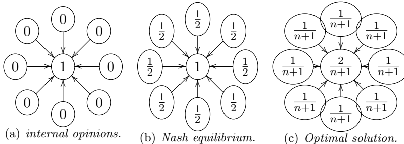
Figure 2: An example demonstrating the price of anarchy of a directed graph can be unbounded.
