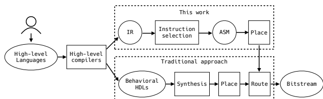
Figure 1. Overview of the traditional compilation pipeline compared to Reticle’s. Independent of the source language, FPGA programs today are funneled down to the same abstraction (hardware description languages). This abstraction is not expressive enough to capture high-performance operations available in DSPs, such as SIMD.
