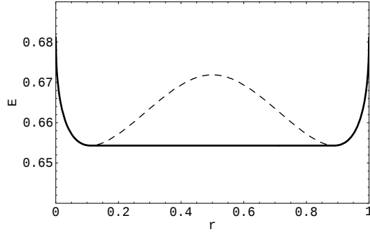
FIG. 3: Entanglement curve for the mixed state \rho_{7;2,5}(r) (full line) constructed as the convex hull of the curve for the pure state |\text{SS}_{7;2,5}(r, \phi)\rangle (dashed in the middle; full at the edges).
