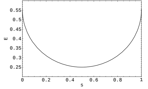
FIG. 1: Entanglement of the pure state \sqrt{s}|W\rangle + \sqrt{1-s}|\widetilde{W}\rangle vs. s . This also turns out to be the entanglement curve for the mixed state s|W\rangle\langle W| + (1-s)|\widetilde{W}\rangle\langle \widetilde{W}| .
