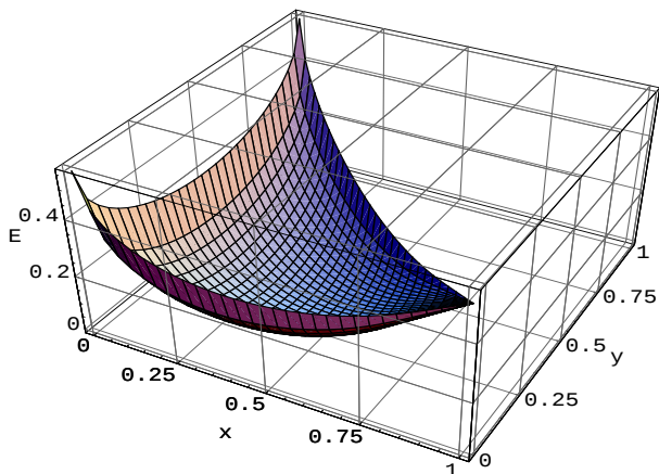
FIG. 9: Entanglement of the mixed state \rho(x, y) .
