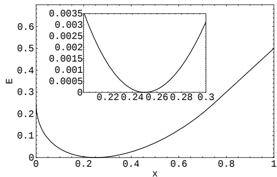
FIG. 10: Entanglement of the mixed state \rho(x, y = (1-x)/2) = x |\text{GHZ}\rangle\langle\text{GHZ}| + \frac{1-x}{2}(|W\rangle\langle W| + |\bar{W}\rangle\langle\bar{W}|) vs. x . Inset: enlargement of the region x \in [0.2, 0.3] . This contains the only point, (x, y) = (1/4, 3/8) , at which E_\rho(x, y) vanishes.
