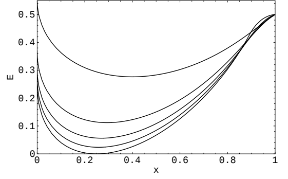
FIG. 8: Entanglement of the pure states |\psi(x, (1-x)r)\rangle = \sqrt{x}|\text{GHZ}\rangle + \sqrt{(1-x)r}|\text{W}\rangle + \sqrt{(1-x)(1-r)}|\widetilde{\text{W}}\rangle vs. x for various values of r (from the top: 0, 0.1, 0.2, 0.3, 0.5). This reveals the nonconvexity in x in the (approximate) interval [0.85, 1] .
