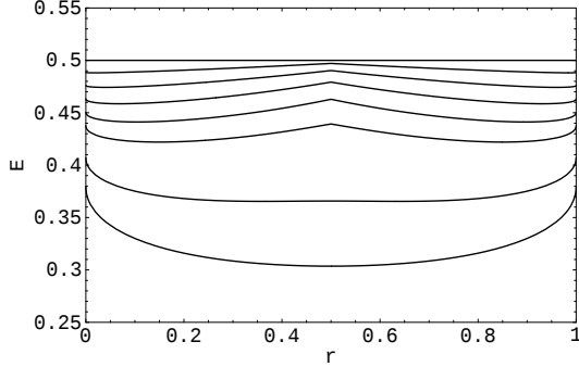
FIG. 7: Entanglement of the pure states |\psi(x, (1-x)r)\rangle = \sqrt{x}|\text{GHZ}\rangle + \sqrt{(1-x)r}|\text{W}\rangle + \sqrt{(1-x)(1-r)}|\widetilde{\text{W}}\rangle vs. r for various values of x (from the bottom: 0.8, 0.85, 0.9, 0.92, 0.94, 0.96, 0.98, 1). This reveals the nonconvexity in r for intermediate values of x .
