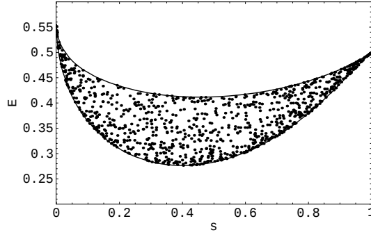
FIG. 2: Entanglement of |\text{GW}(s, \phi)\rangle vs. s . The upper curve is for \phi = \pi whereas the lower one is for \phi = 0 . Dots represent states with randomly generated s and \phi .
