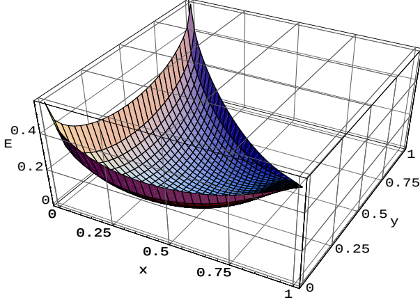
FIG. 4: Entanglement vs. the composition of the pure state |\psi(x, y)\rangle . This entanglement surface is not convex near (x, y) = (1, 0) , although not obvious from the plot.
