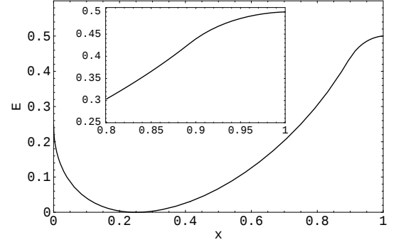
FIG. 5: Entanglement of the pure state |\psi(x, y = (1-x)/2)\rangle = \sqrt{x} |\text{GHZ}\rangle + \sqrt{(1-x)/2} |\text{W}\rangle + \sqrt{(1-x)/2} |\widetilde{\text{W}}\rangle vs. x . This shows the entanglement along the diagonal boundary x + 2y = 1 . Note the absence of convexity near x = 1 ; this region is repeated in the inset.
