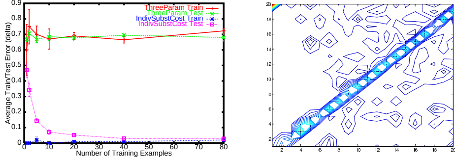
Figure 4: Left: Train and test error rates for the 3 and the 403 parameter model depending on the number of training examples. Right: Typical learned substitution matrix after 40 training examples for the 403-parameter model.
