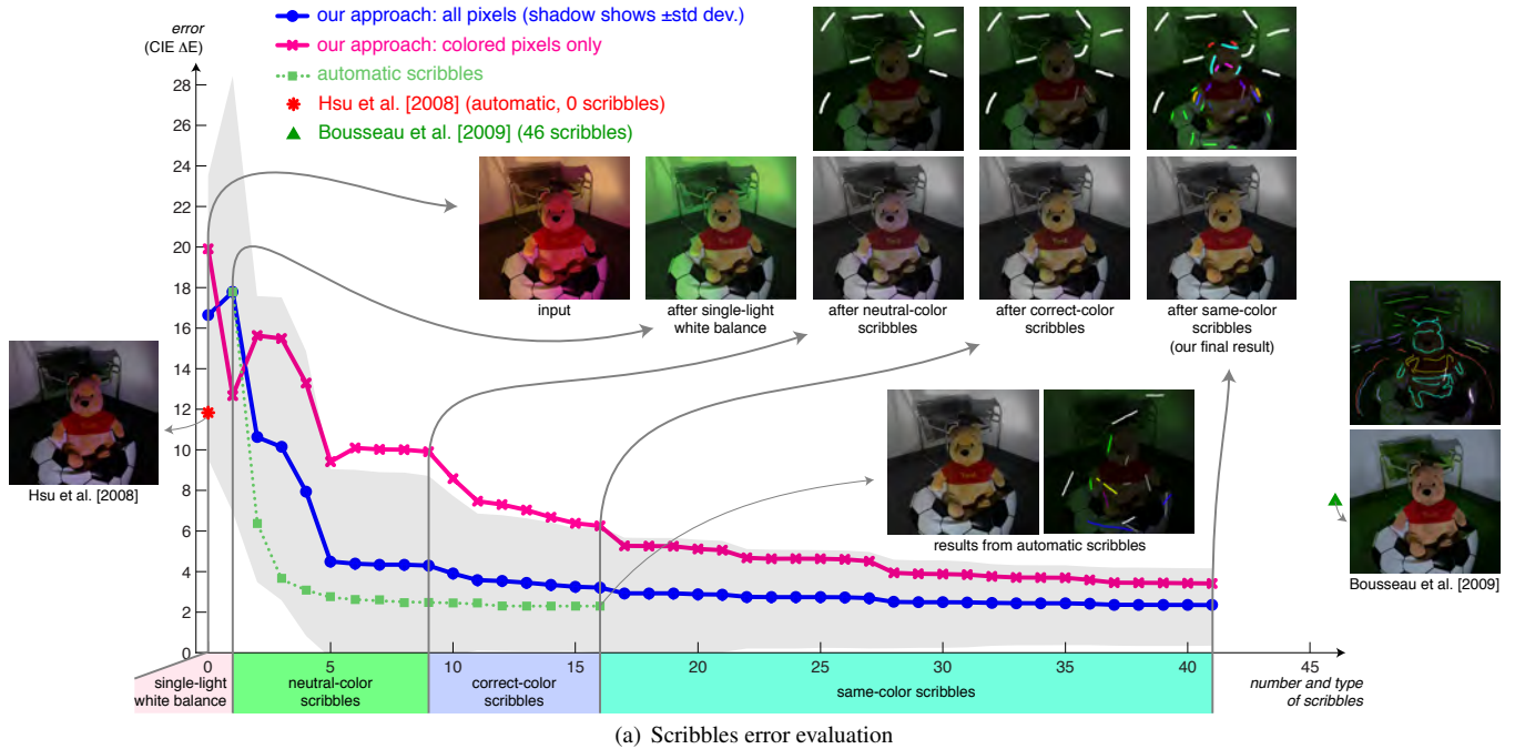
Figure 5: We evaluated the effect of our scribbles on the semi-synthetic image (Fig. 4). The use of neutral scribbles alone fixes the gray floor and the white wall, but extrapolates wrong colors elsewhere. By adding correct-color scribbles to fix a few of the natural looking colors, produced by the single-light white balance stage, we get better looking regions. Finally, we introduce a couple of same-color scribbles to propagate correct color information to other parts of the image. The solution produced by our system is free of color casts, visually (Fig. 4h) and numerically closer to the ground truth, compared to the methods of [Bousseau et al. 2009] and [Hsu et al. 2008].
