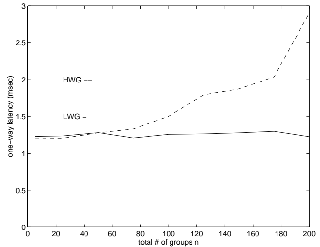
Figure 12. Data transfer
