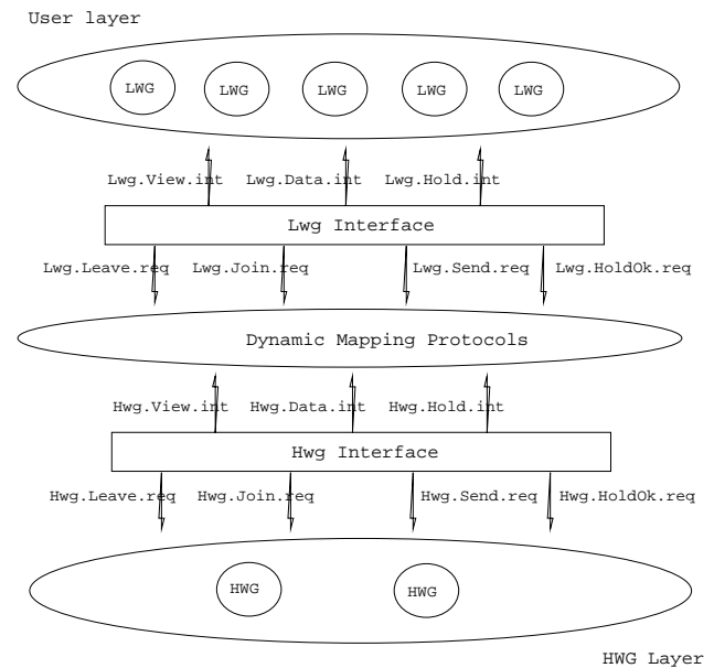
Figure 1. Light-Weight Group service interface
