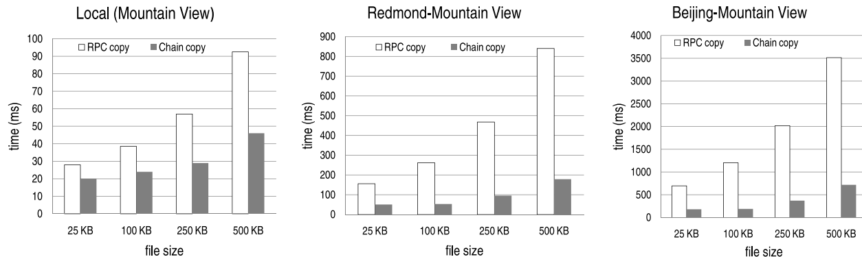
Figure 10: Comparison of RPC copy and Chain copy under various settings. (Left) Client and servers are in the same site in Mt. View. (Center) Client is in Redmond and servers are in Mt. View. (Right) Client is in Beijing and servers are in Mt. View.
