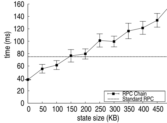
Figure 9: Execution time using an RPC chain versus standard RPC to call 2 servers.
