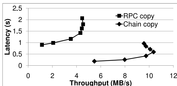
Figure 11: Throughput-latency of RPC copy and Chain copy. Latency is the time to copy a 128 KB file, and throughput is the rate at which files are copied.
