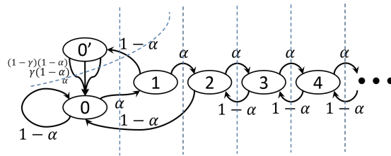
Fig. 4: State machine with transition frequencies and analysis cuts.
