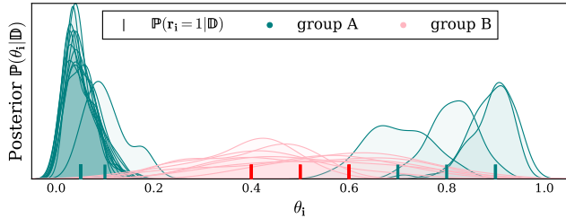
Figure 3: An illustration of disparate uncertainty between groups from a Bayesian perspective for all the candidates of Figure 1. The candidates in group A have peaked posteriors, while those in group B have relatively flat posteriors.
