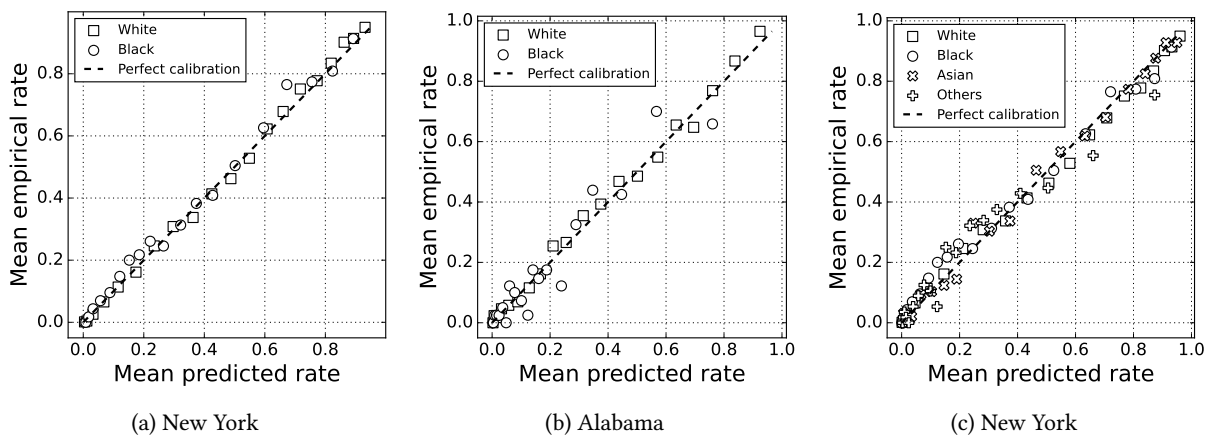
Figure 12: Calibration plot for \mathbb{P}(r_i|\mathcal{D}) for the state of New York and Alabama
