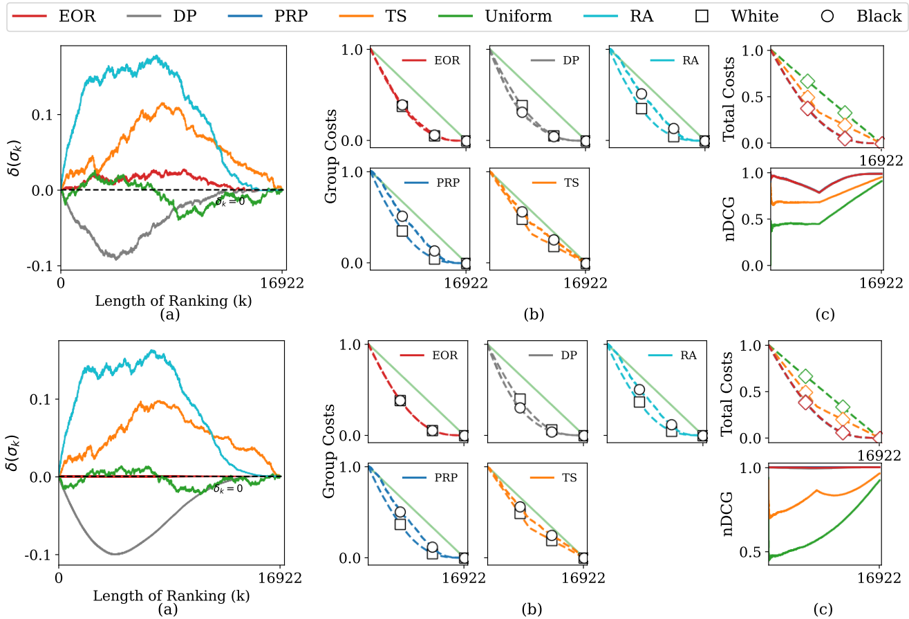
Figure 14: Top: EOR criterion \delta(\sigma_k) and Costs computed using true relevance labels \sigma_k from the test subset. Bottom: EOR criterion \delta(\sigma_k) and Costs computed using calibrated \mathbb{P}(r_i|\mathcal{D}) for the state of New York.
