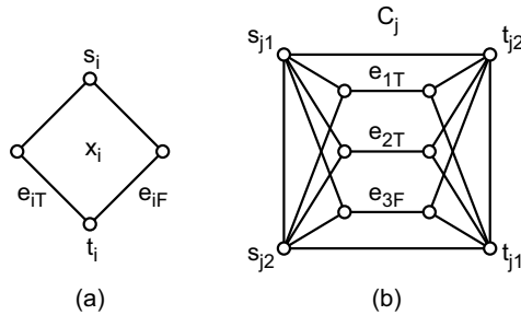
Figure 6: Gadgets for the NP-completeness reduction.
