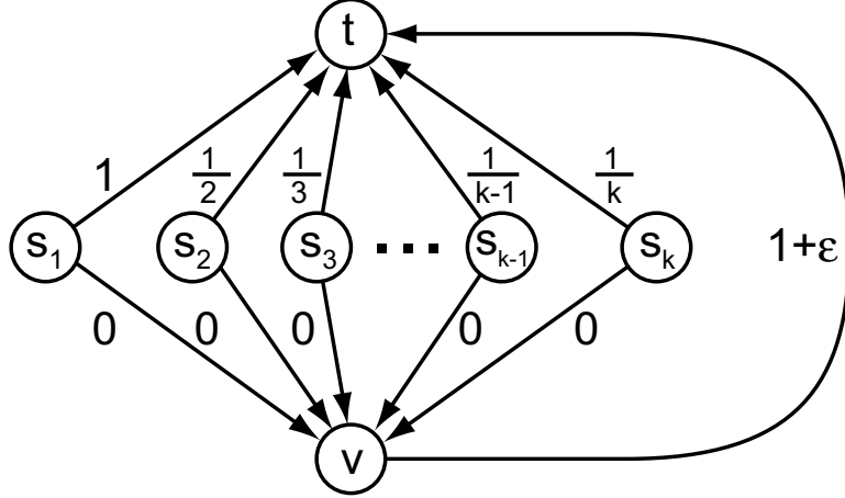
Figure 1: An instance in which the price of stability converges to H(k) = \Theta(\log k) as \varepsilon \rightarrow 0 .
