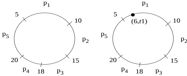
Figure 2: Mapping Ranges to Peers
