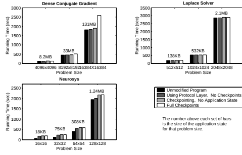
Fig. 5. Point-to-point Overheads
