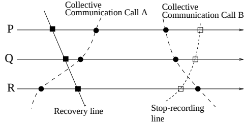
Fig. 4. Collective Communication
