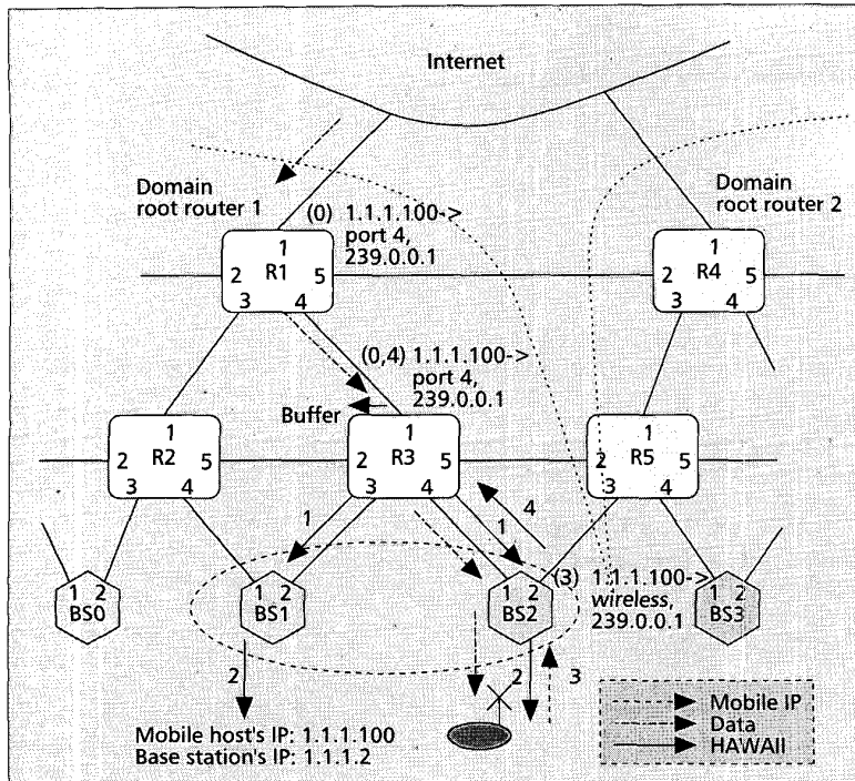
■ Figure 5. Paging.
