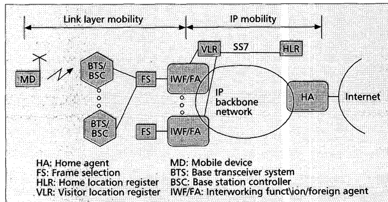
■ Figure 2. CDMA network architecture.
