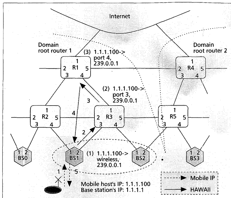
■ Figure 3. Power-up.
