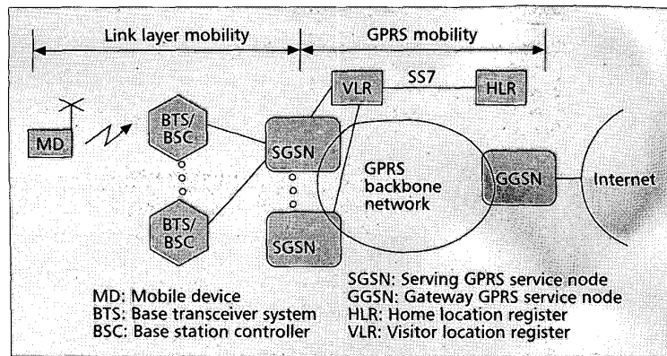
■ Figure 1. GPRS network architecture.
