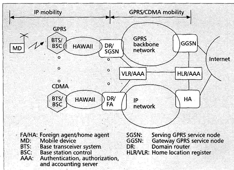
■ Figure 9. HAWAII in the access network.
