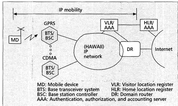
■ Figure 8. The HAWAII-based architecture.
