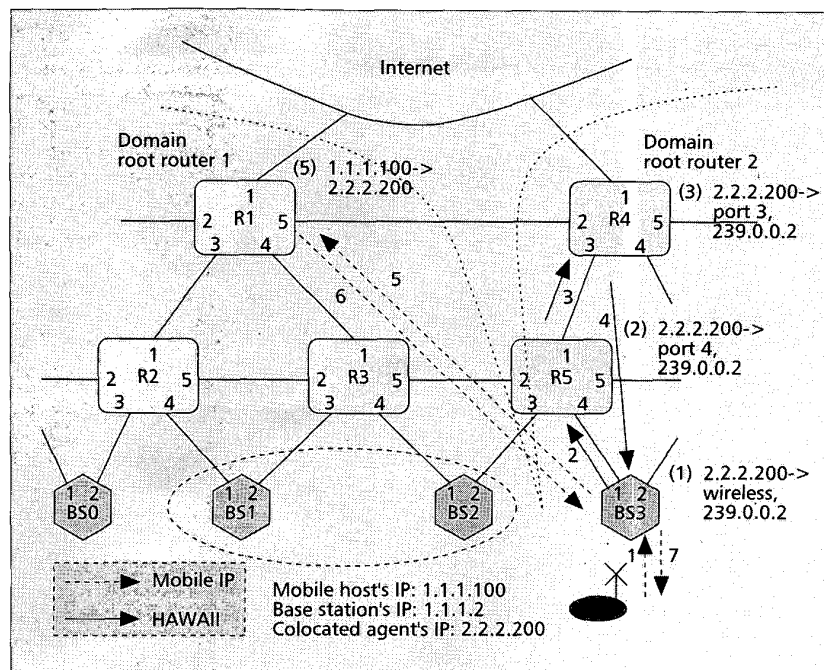
Figure 6. Interdomain handoff.
