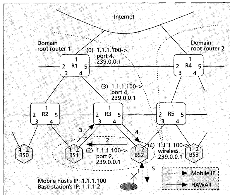
Figure 4. Intradomain handoff.
