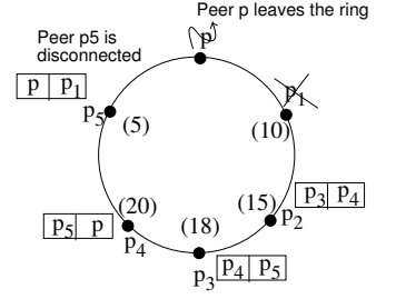
Figure 14. Naive merge leads to reduced reliability
