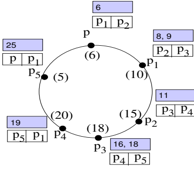
Figure 8. Peer p just inserted into the system
