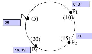
Figure 3. Data Store
