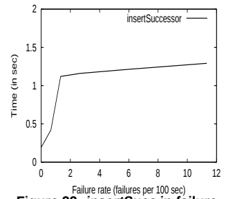
Figure 23. insertSucc in failure mode
