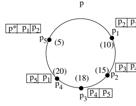
Figure 11. After p_5.\text{insertSucc} call
