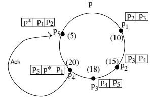
Figure 12. Propagation and final ack
