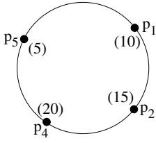
Figure 2. Ring
