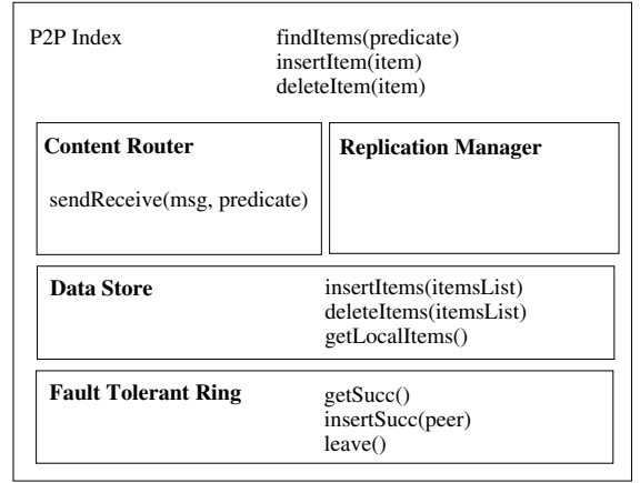
Figure 1. Indexing Framework
