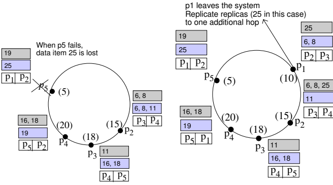
Figure 17. Peer p_5 fails causing loss of item 25
