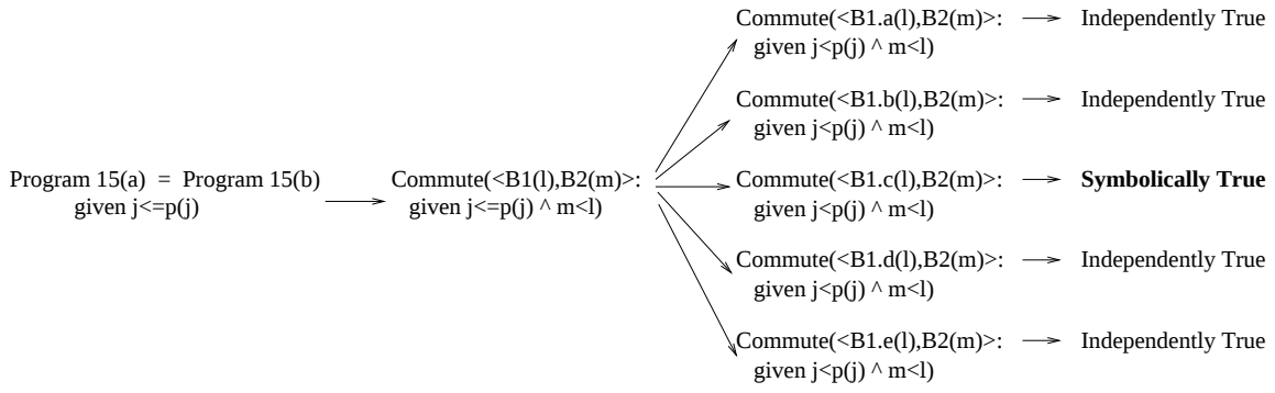
Figure 17: Commute Calls for LU
