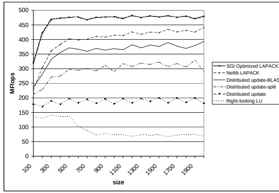
Figure 20: Transforming LU with Pivoting
