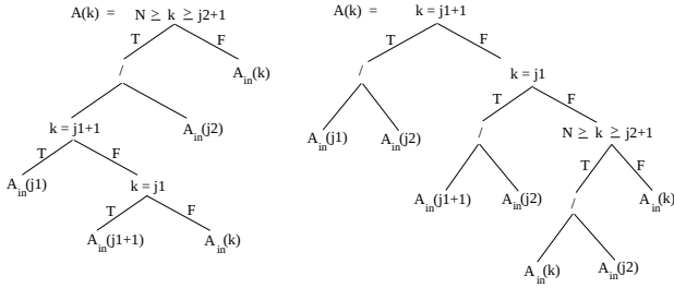
(a) Tree for Figure 3(d) (b) Tree for Figure 3(e)
