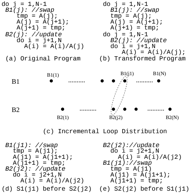
Figure 3: Loop Distribution in Running Example
