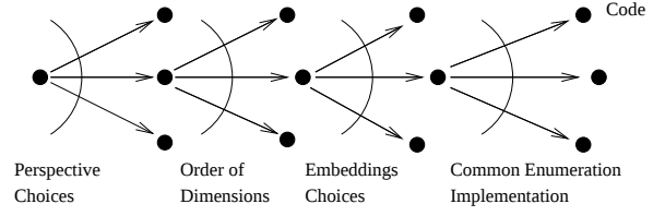
Figure 10: Search Space
