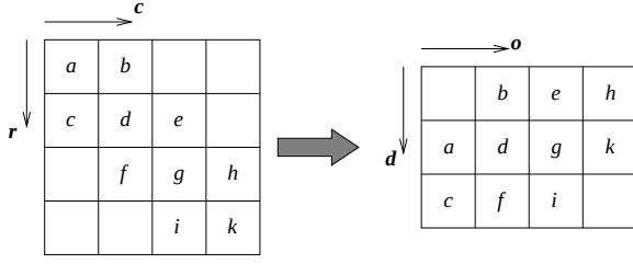
Figure 2: DIA Storage Format
