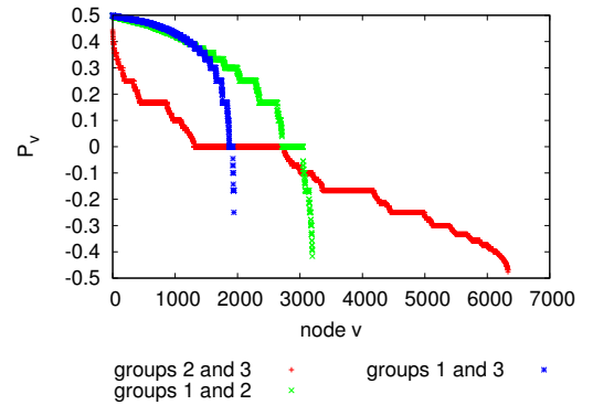
Figure 5: Distribution of P_v for communities debating Gun Control. On the pairs of polarized communities (1–2 and 1–3), few nodes establish more connections with the alternate group than with internal nodes ( P_v < 0 ).
