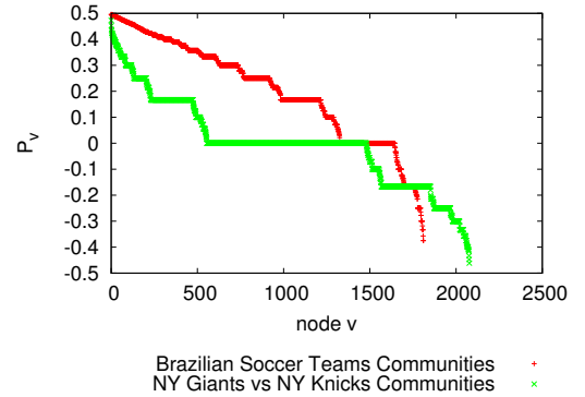
Figure 3: Distribution of P_v for Twitter communities debating Sports. A polarized social network is characterized by a small number of nodes preferring cross-boundary connections ( P_v < 0 ).
