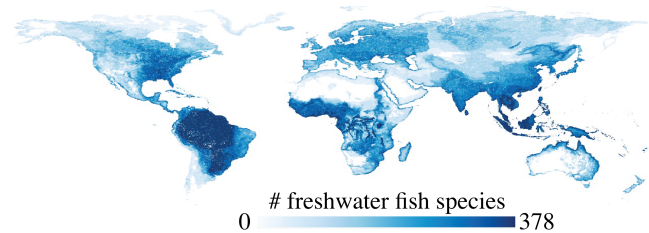
Figure 1: The global distribution of freshwater fish species richness (total of 13,740 species), where color saturation indicates the number of species in each hydrological unit (total of 190,675 units).
