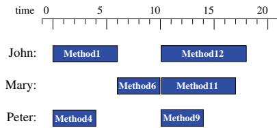
Figure 2: The optimal schedule for the agents corresponding to the problem of Figure 1, with total quality 34.
