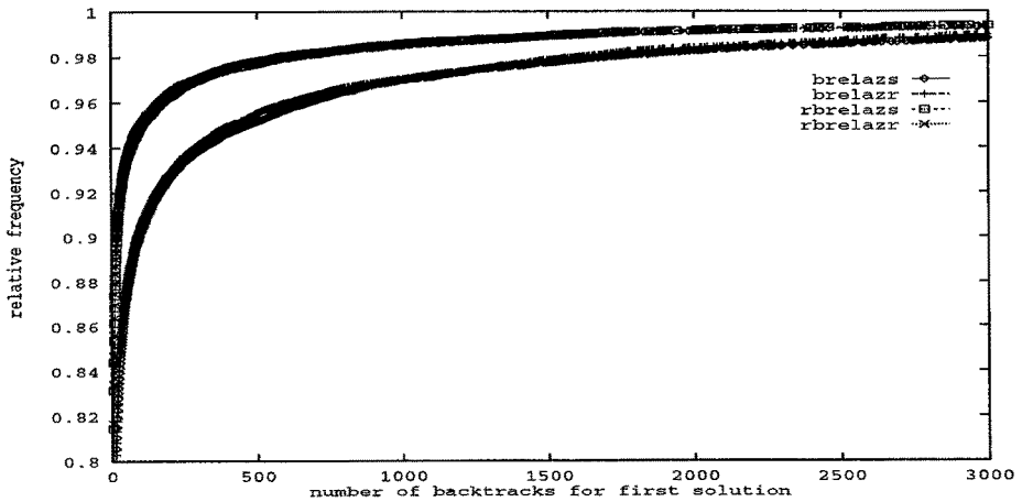
Figure 5: Finding quasigroups of order 10 at the phase transition.
