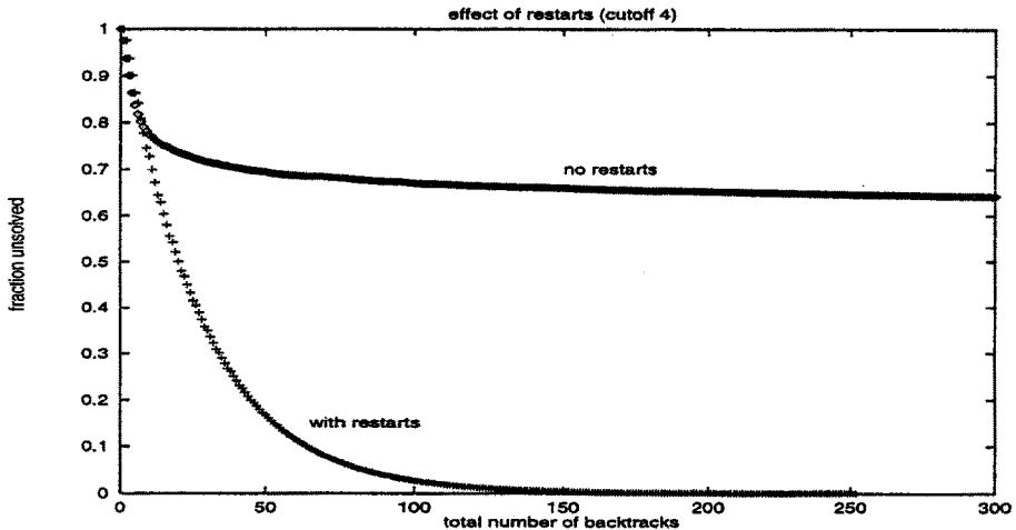
Figure 8a: Using restarts to exploit heavy-tailed behavior.
