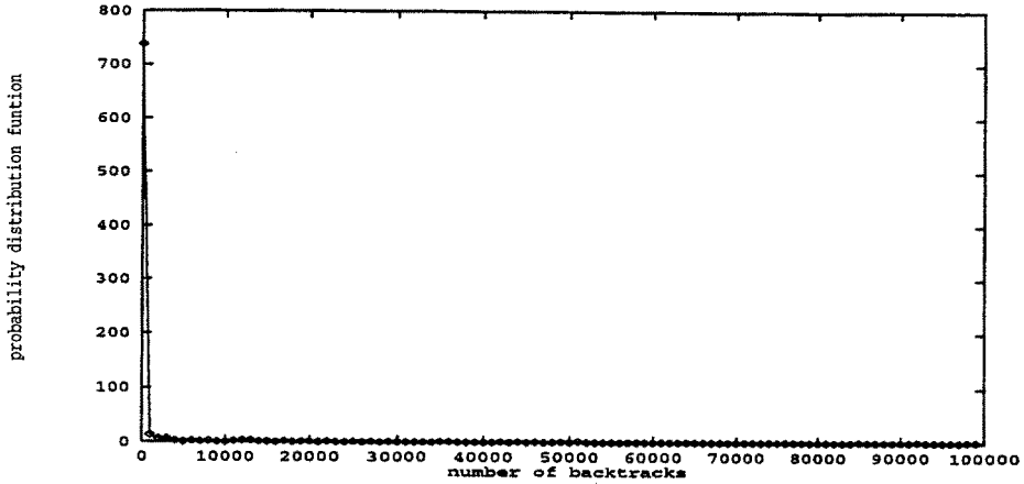
Figure 6a: Probability distribution exhibiting heavy-tailed behavior.
