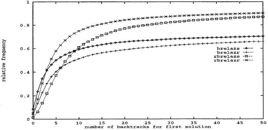
Figure 4: Finding quasigroups of order 20 with 10% pre-assigned values.
