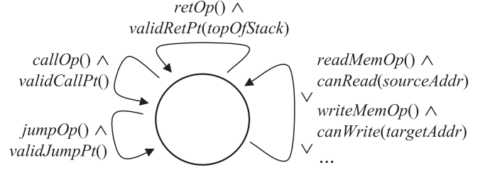
Figure 5. A security automaton for SFI-like memory protection
