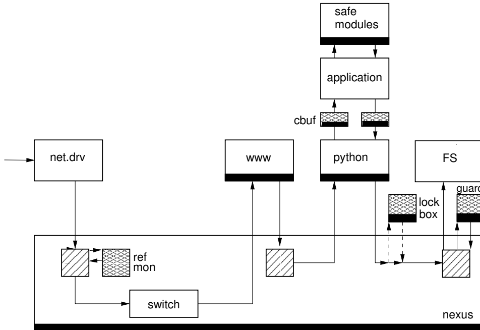
Figure 3: The Fauxbook multi-tier webservice. Cross-hatched boxes denote enforcement mechanisms, shaded boxes identify decision caches and thick borders indicate hash attestation.
