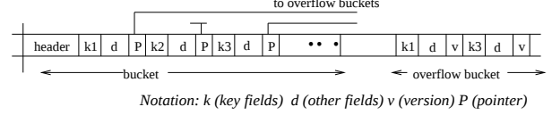
Figure 1. Multiversion broadcast
