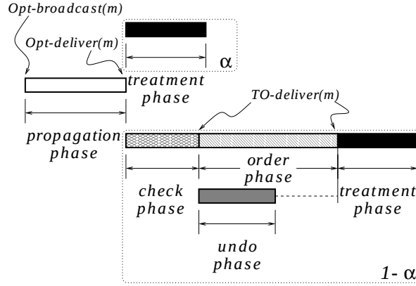
Figure 5.5: Hybrid approach
