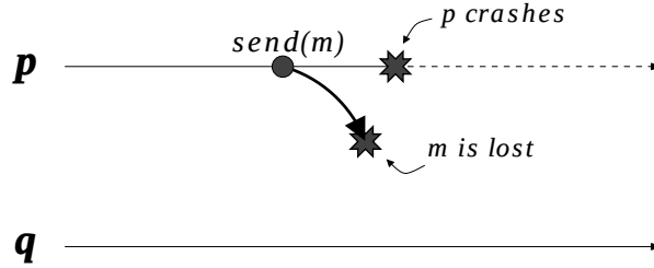
Figure 2.1: Quasi-Reliable Channels
