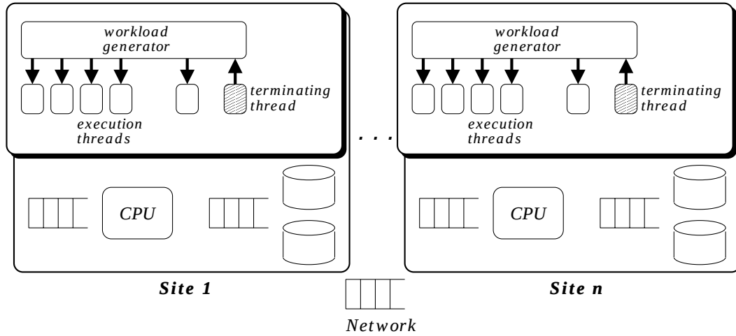
Figure 3.6: Simulation model
