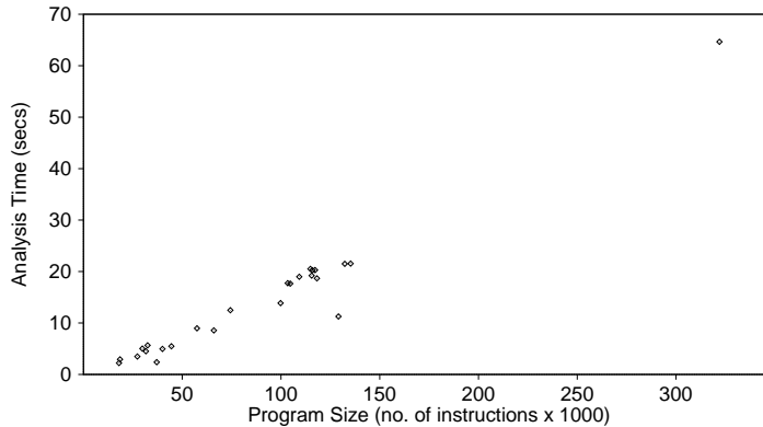
Figure 4: Variation of analysis time with input size
