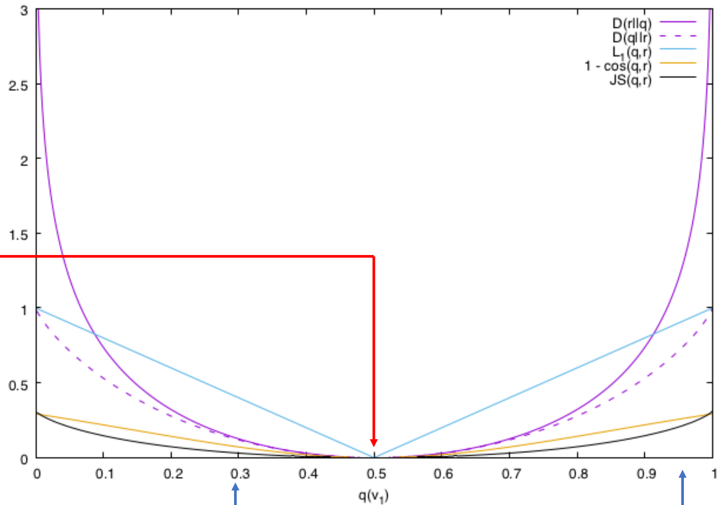
Distances between distributions q and fixed r , where r(v_1) = r(v_2) = .5 (Variation on Figure 2.1 of Lee 1997 PhD thesis)
