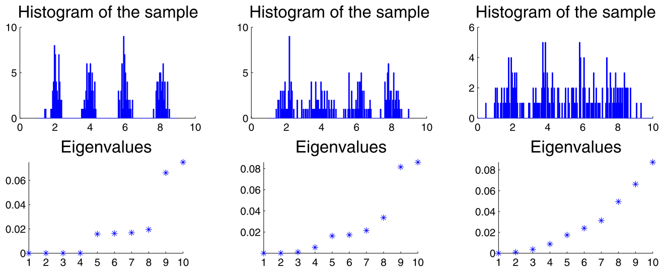
Fig. 4 Three data sets, and the smallest 10 eigenvalues of L_{TW} . See text for more details
