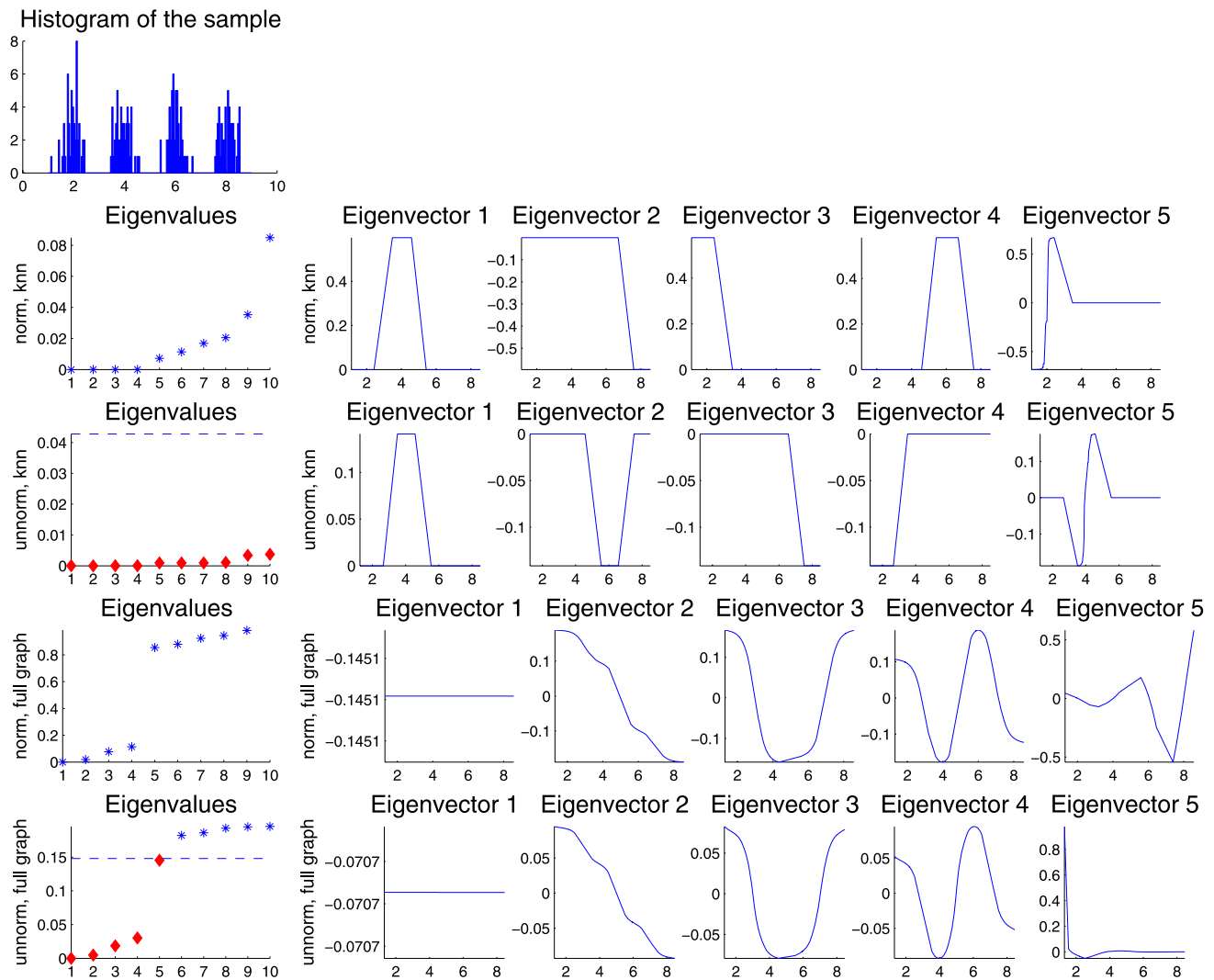
Fig. 1 Toy example for spectral clustering where the data points have been drawn from a mixture of four Gaussians on \mathbb{R} . Left upper corner : histogram of the data. First and second row : eigenvalues and eigenvectors of L_{TW} and L based on the k -nearest neighbor graph. Third and
