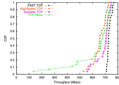
Fig. 12. Overall evaluation: throughput.
