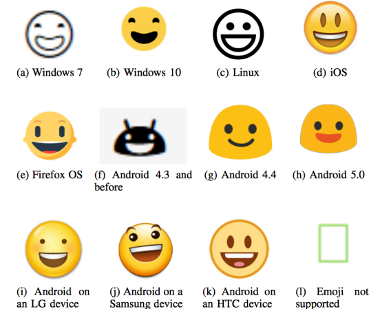
Canvas
