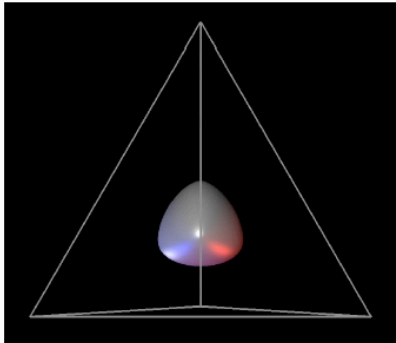
Loop
