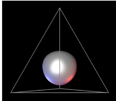
Catmull-Clark
