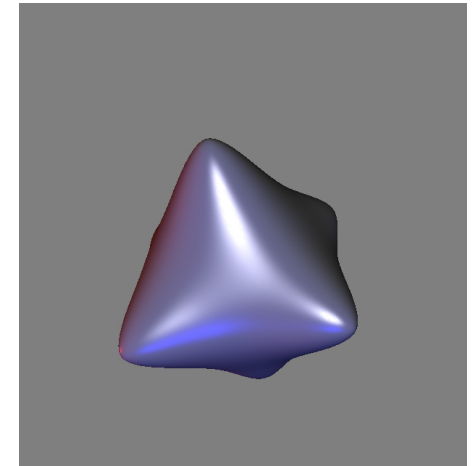
limit surface
