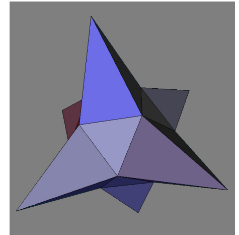
control polyhedron
