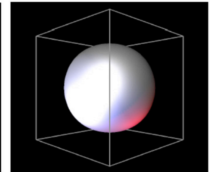
Catmull-Clark
