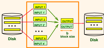
B main memory buffers, k-way merge
