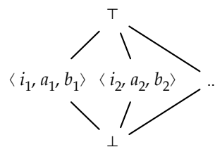
Figure 1: Dataflow values for induction variables analysis
