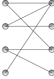
Figure 7.3: Example of a bipartite graph.
