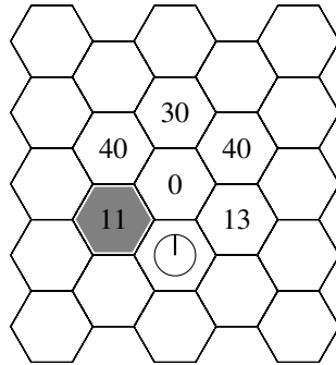
Figure 5: Using ping in a simple environment. The number on each hex represents a valid value for ping if that hex had the only food in the world.
