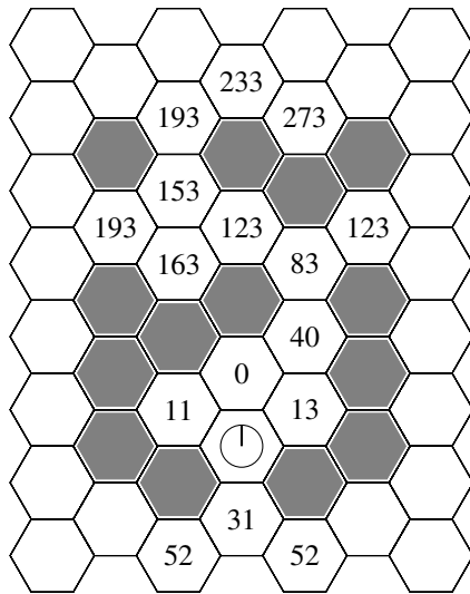
Figure 6: Using ping in a challenging environment. The number on each hex represents a valid value for ping if that hex had the only food in the world.
