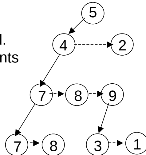
Tree represented using GTreeCell
