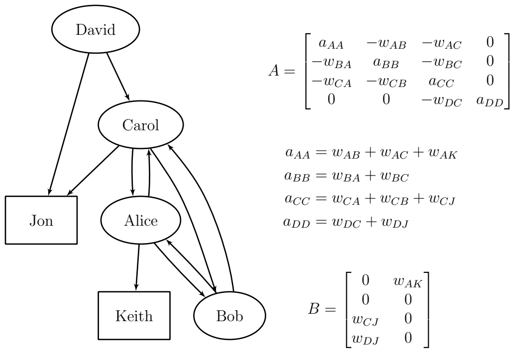
Figure 1: Small example of opinion formation in a social network. If Alice, Bob, Carol, and David have opinions x_A, x_B, x_C, x_D and Jon and Keith have opinions y_J and y_K , then we compute x_A through x_D using the matrix equation Ax = By .
