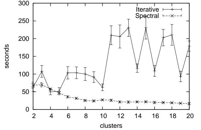
Figure 2: Training time versus number of clusters in each example.
