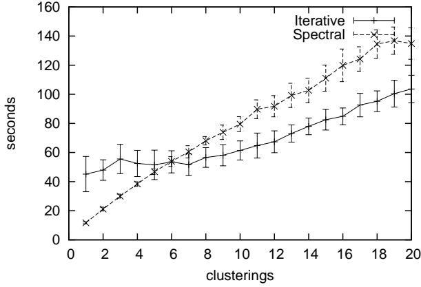
Figure 1: Training time versus number of example clusterings in the training set.
