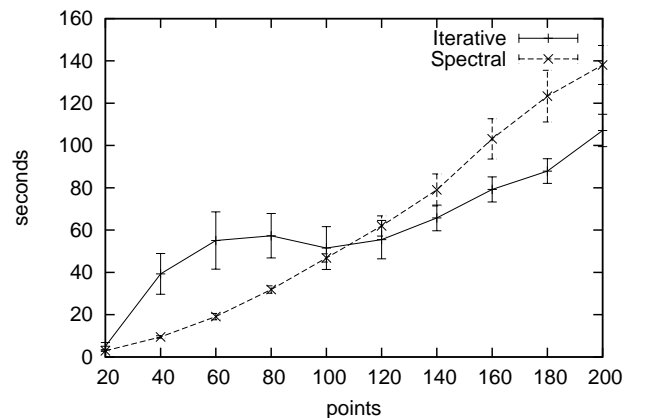
Figure 4: Training time versus number of points.
