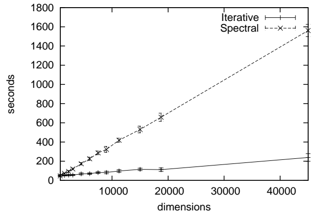
Figure 3: Training time versus number of features.
