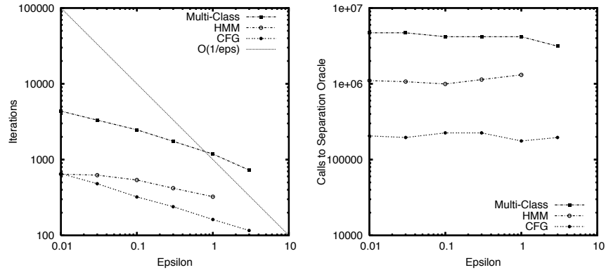
Fig. 7 Number of iterations for the 1-slack algorithm (left) and number of calls to the separation oracle for the 1-slack algorithm with caching (right) as a function of \epsilon at the maximum training set size.
