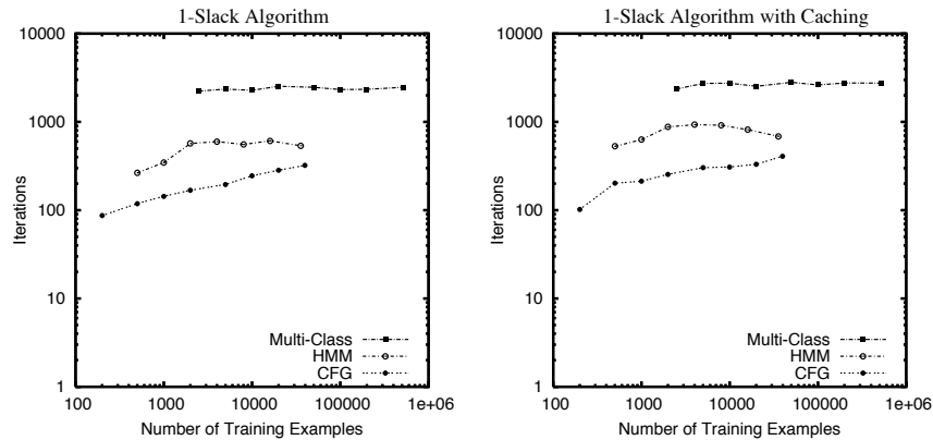
Fig. 2 Number of iterations as a function of n for the 1-slack algorithm (left) and the 1-slack algorithm with caching (right).
