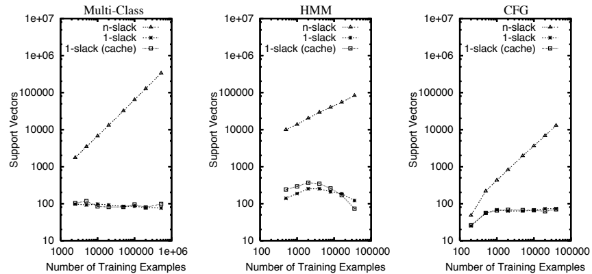
Fig. 3 Number of support vectors for multi-class classification (left) HMM part-of-speech tagging (middle) and CFG parsing (right) as a function of n for the n -slack algorithm, the 1-slack algorithm, and the 1-slack algorithm with caching.
