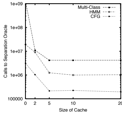
Fig. 5 Number of calls to the separation oracle as a function of cache size for the the 1-slack algorithm (right).
