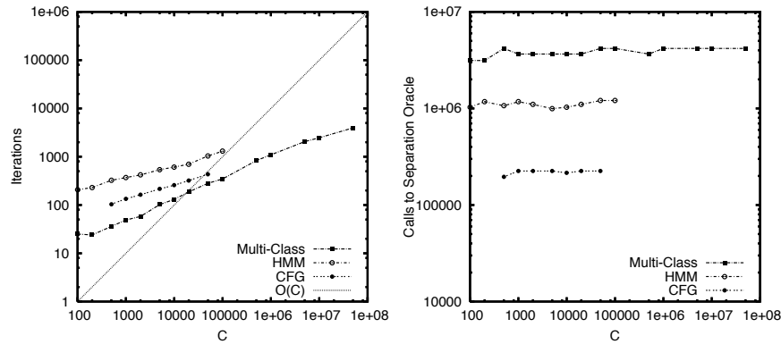
Fig. 8 Number of iterations for the 1-slack algorithm (left) and number of calls to the separation oracle for the 1-slack algorithm with caching (right) as a function of C at the maximum training set size.
