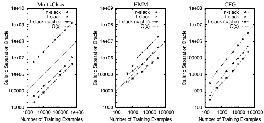
Fig. 4 Number of calls to the separation oracle for multi-class classification (left) HMM part-of-speech tagging (middle) and CFG parsing (right) as a function of n for the n -slack algorithm, the 1-slack algorithm, and the 1-slack algorithm with caching.
