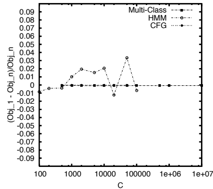
Fig. 6 Relative difference in dual objective value of the solutions found by the 1-slack algorithm and by the n -slack algorithm as a function of C at the maximum training set size.
