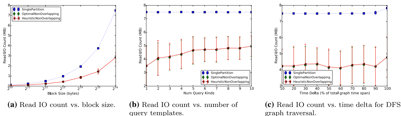
Fig. 10 Experiments on real Twitter data show the benefits in terms of IO cost for the RailwayDB adaptive storage system. a Read IO count versus block size, b Read IO count versus number of query templates, c Read IO count versus time delta for DFS graph traversal
