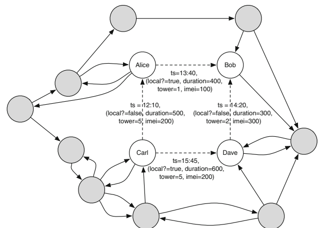
Fig. 1 A partial example interaction graph for call data records, capturing the telephone calls among a set of people. The running example focuses on a subgraph indicated by the nodes colored white . Each edge in the graph is associated with attributes for the interaction, including the time the call was placed, whether the call was local, the duration of the call, the cell phone tower, and the IMEI number identifying the device used
