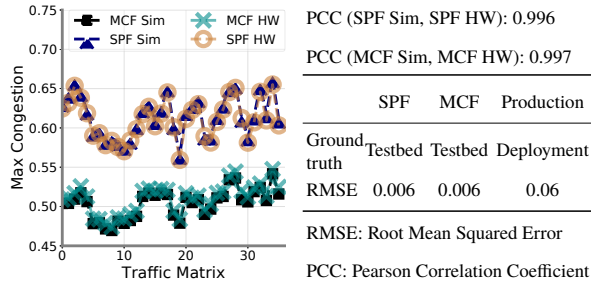
Figure 8: Calibration: simulator vs. SDN testbed and LBN.
