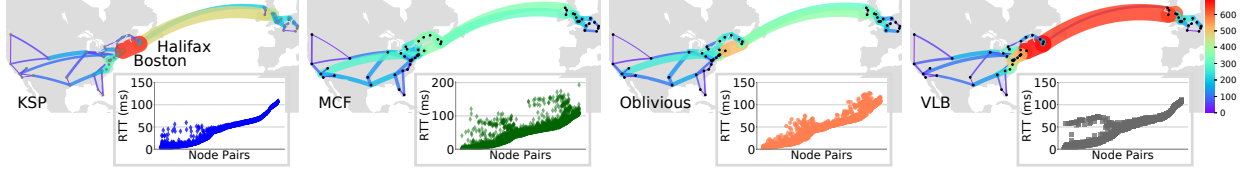
Figure 4: Figure showing sum of path weights for each link, for different path-selection algorithms. Inset shows length of paths selected by each algorithm for different node pairs. x -axis has node pairs sorted by their geographical distances.
