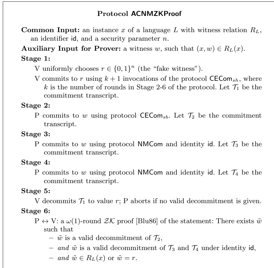
Fig. 1. An Adaptive Concurrent Non-Malleable \mathcal{ZK} Proof for \mathcal{NP}
