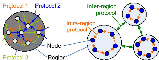
Figure 5: QuickSilver amortizes costs over many groups. Lacking such an approach, chaos can occur, as is seen on the left, where each group builds its own recovery infrastructure (here, a tree-like overlay).
