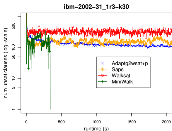
Figure 3: Qualitative search behavior in terms of the number of unsatisfied clauses (y-axis, log scale) vs. runtime (x-axis). Both state-of-the-art pure local search methods, unguided Walksat and MiniWalk are shown. Note the unique steep drops of MiniWalk. Instance: ibm-2002-31_1r3-k30.cnf .
